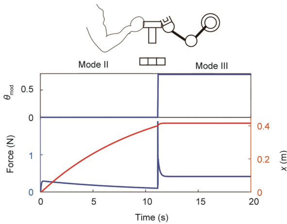
Fig. 9. The interaction force and displacement of the robot when the switch mode is based on the task requirement.
