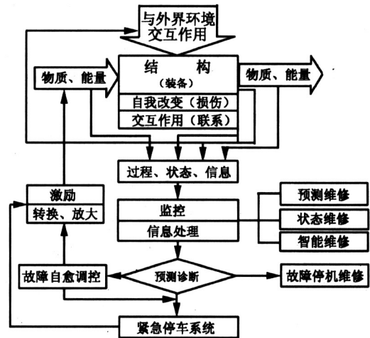
图 3 故障自愈调控系统 (FSR) 模式简图 Fig.3 Scheme of faults self-recovering and controlling
