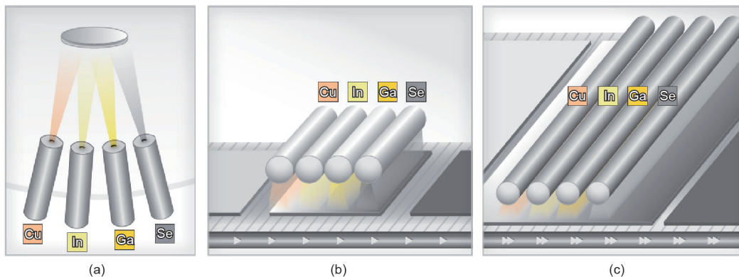
Fig. 3. Configurations for CIGS deposition by co-evaporation. (a) Static configuration, in which fluxes are regulated over time; (b) inline configuration, in which sources are configured to provide correct constant fluxes to a moving substrate; (c) industrial configuration, which coats larger substrates at faster speeds.
