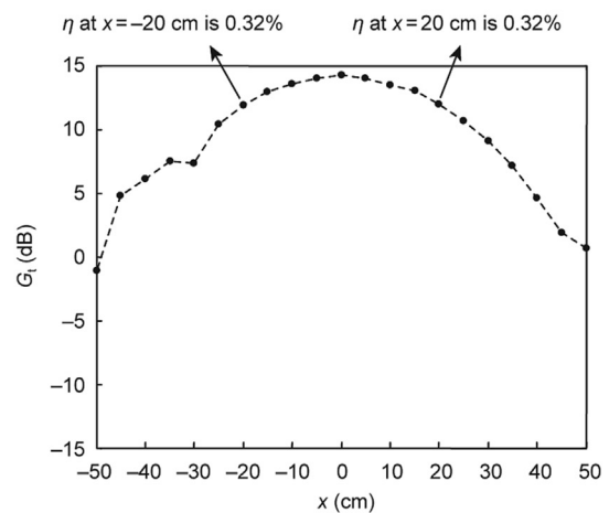
Fig. 7. Experimental results with two targets broadcasting CW pilot signals of the same frequency at 5.75 GHz. The phase difference between the excitations of two pilot signals is about 0.
