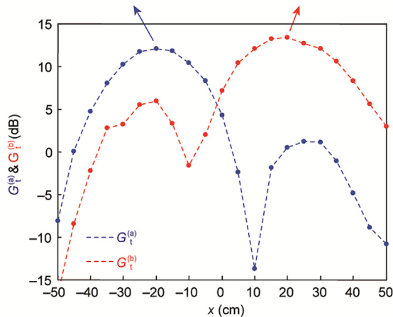
Fig. 6. Experimental results with two targets broadcasting CW pilot signals of 5.745 and 5.755 GHz respectively. G_t^{(a)} : the antenna gain of the four-element array at frequency f^{(a)} = 5.745 GHz; G_t^{(b)} : the antenna gain of the four-element array at frequency f^{(b)} = 5.755 GHz.
