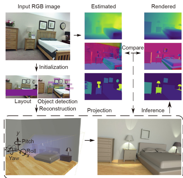
Fig. 6. Illustration of 3D indoor scene parsing and reconstruction in an analysis-by-synthesis fashion [36]. A 3D representation is initialized by individual vision tasks (e.g., object detection, 2D layout estimation). A joint inference algorithm compares the differences between the rendered normal, depth, and segmentation maps and the ones estimated directly from the input red-green-blue (RGB) image, and adjusts the 3D structure iteratively. Reproduced from Ref. [36] with permission of Springer, ©2018.
