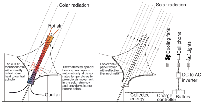
Fig. 5. A combination of solar collection and solar chimneys make air movement possible on a very low-tech system. The umbrella is moved to appropriate angles by the occupants of the kiosk who are seeking shade. (Image courtesy of DOSU Studio Architecture.)
