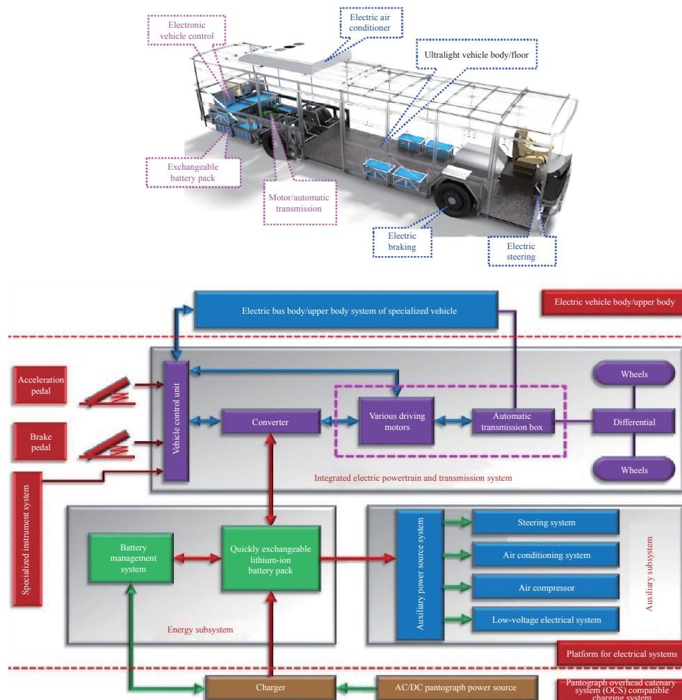
Fig. 2. Configuration of a highly efficient electric bus powertrain system.
