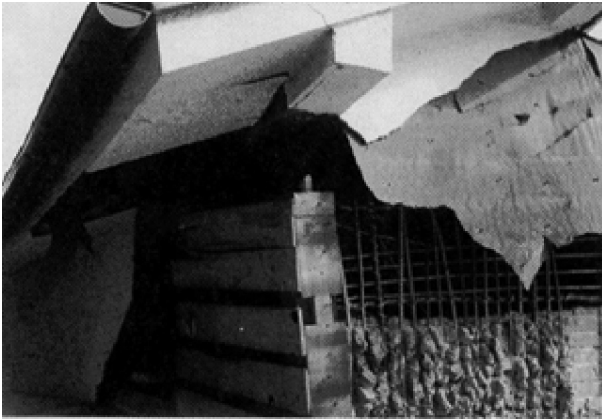
Fig. 8. Connection failure of a wooden house in the Great Hanshin earthquake in 1995 [8].
