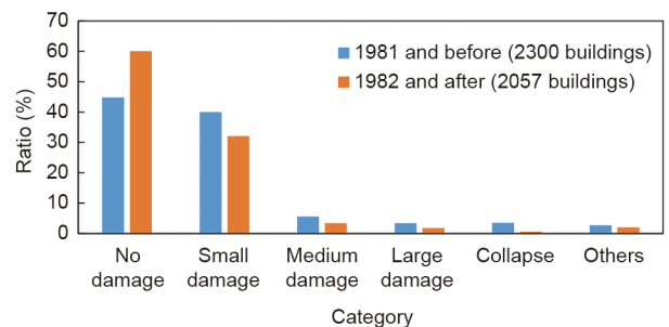
Fig. 10. Percentages of damaged buildings in the Great Hanshin earthquake [6].
