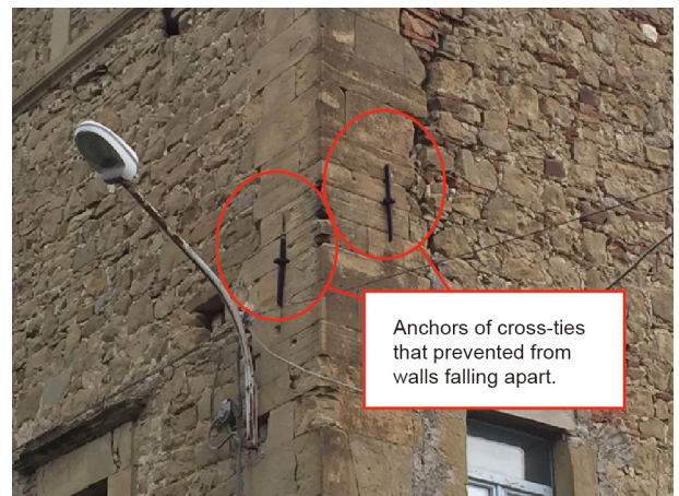
Fig. 4. Surviving masonry building with cross-tie reinforcement in the Amatrice earthquake.
