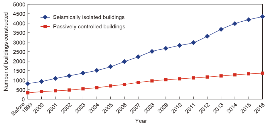
Fig. 16. Statistics of seismically isolated and passively controlled buildings in Japan.
