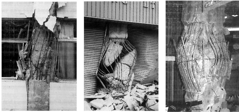
Fig. 6. Failure of RC columns in the Great Hanshin earthquake in 1995 [6].
