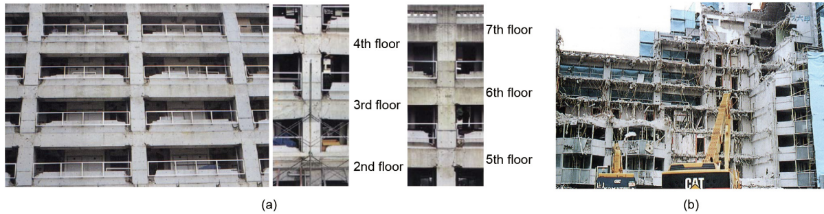
Fig. 11. Damaged and demolished residential buildings in the Great Hanshin earthquake. (a) Flexural cracks of beams; (b) demolished building.
