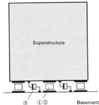
Fig. 15. Schematic diagram of a seismically isolated structure. The superstructure is flexibly connected to the foundations by mechanisms ①, ②, and ③, where mechanism ① supports the superstructure in the vertical direction, mechanism ② exhibits a restoring force in the horizontal direction, and mechanism ③ absorbs energy in the relative displacement between the superstructure and the foundations [9].
