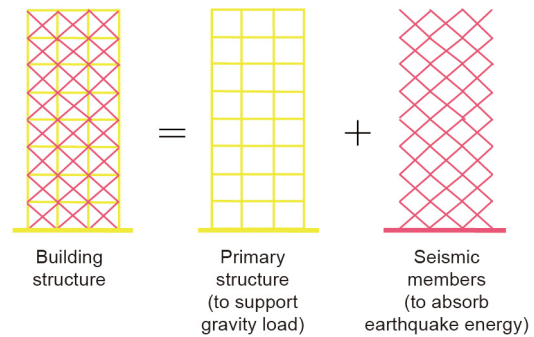
Fig. 14. Separation of primary and seismic members in an alternative approach to ductility design.
