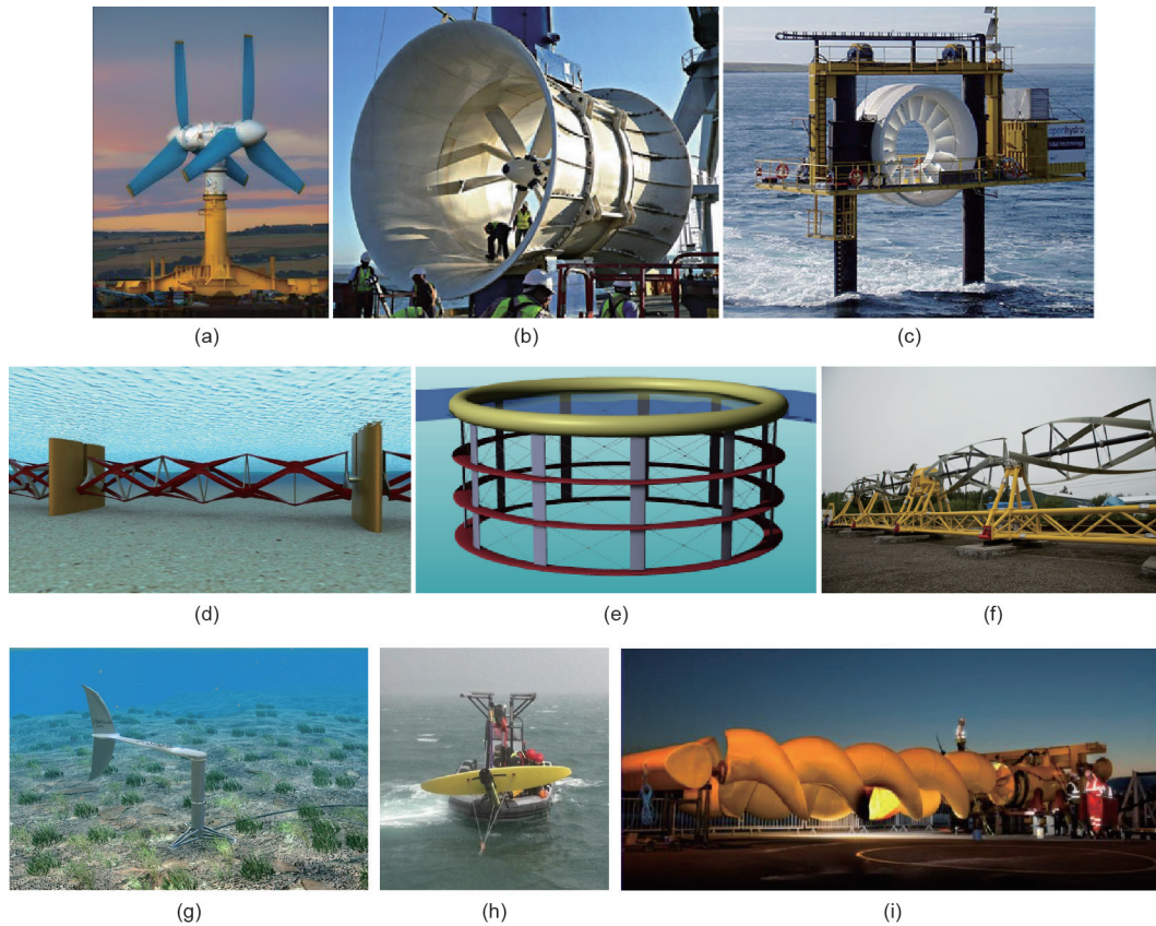
Fig. 4. Examples of tidal and ocean current devices. (a) Atlantis AK1000 axial-flow turbine (1 MW) [31]; (b) Atlantis Solon-K ducted turbine (1 MW) [32]; (c) OpenHydro open-center turbine (250 kW) [33]; (d) Kepler transverse horizontal axis water turbine (THAWT), a kind of cross-flow turbine (4 MW) [34]; (e) Edinburgh vertical axis cross-flow turbine concept (100 MW) [35]; (f) Gorlov helical turbines before deployment at Cobscook Bay, ME, USA [36]; (g) bioSTREAM (150 kW) oscillatory-hydrofoil turbine (image courtesy of BioPower) [37]; (h) Minesto deep sea tidal kite [38]; (i) Flumill Archimedes screw turbine [39].
