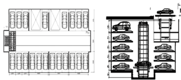
Fig. 6. Aisle-stack mechanical parking system.
