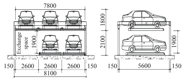
Fig. 11. Design of the space of the parking lot (unit: mm).
