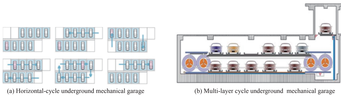
Fig. 5. Types of circulating underground mechanical parking lots.
