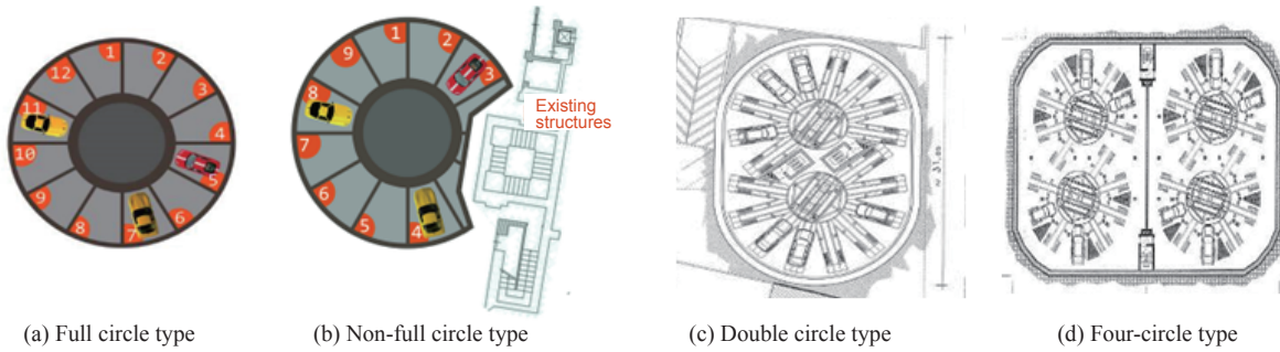
Fig. 4. Types of cylindrical underground parking.
