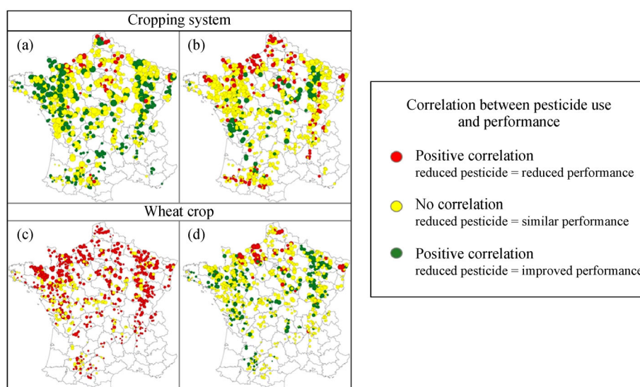
Fig. 1 Mapping of the correlations between pesticide use and productivity (a, c) and profitability (b, d), either computed at the cropping system level (a, b) or at the specific crop (viz. wheat) level (c, d). Adapted from Lechenet et al. [17] , with permission from Springer Nature.
