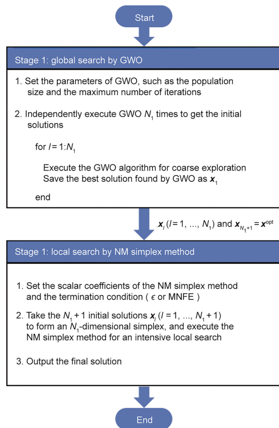
Fig. 3. Diagram of the GWO–NM method.
