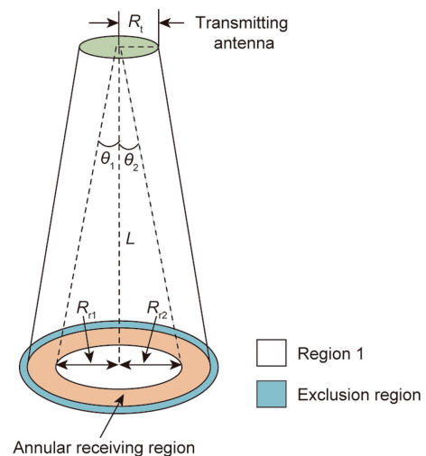
Fig. 1. Illustration of an MPT system with an annular collection area. R_{r1} : the inner radius of the annular receiving area; R_{r2} : the outer radius of the annular receiving area; R_t : the radius of the transmitting antenna; L : the distance between the transmitting antenna and rectenna; \theta_1, \theta_2 : the angles of the annular receiving area.
