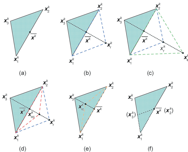
Fig. 2. Illustration on (a) an initial simplex in 2D space and operations of (b) reflection, (c) expansion, (d) outside contraction, (e) inside contraction, and (f) shrinking.
