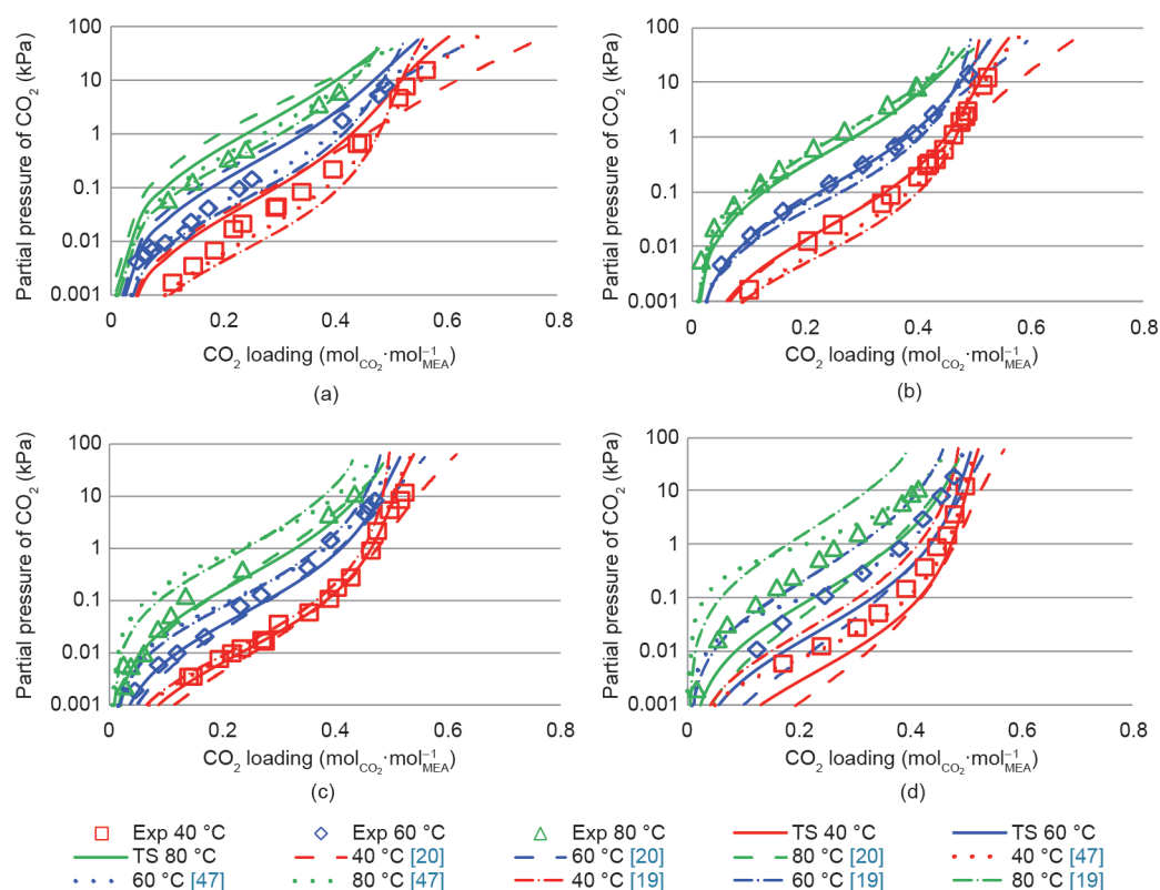
图2. \text{CO}_2 气相分压和液相 \text{CO}_2 载荷的关系: (a) 15 wt% MEA 溶剂; (b) 30 wt% MEA 溶剂; (c) 45 wt% MEA 溶剂; (d) 60 wt% MEA 溶剂。Exp: 实验数据; TS: 本文。
