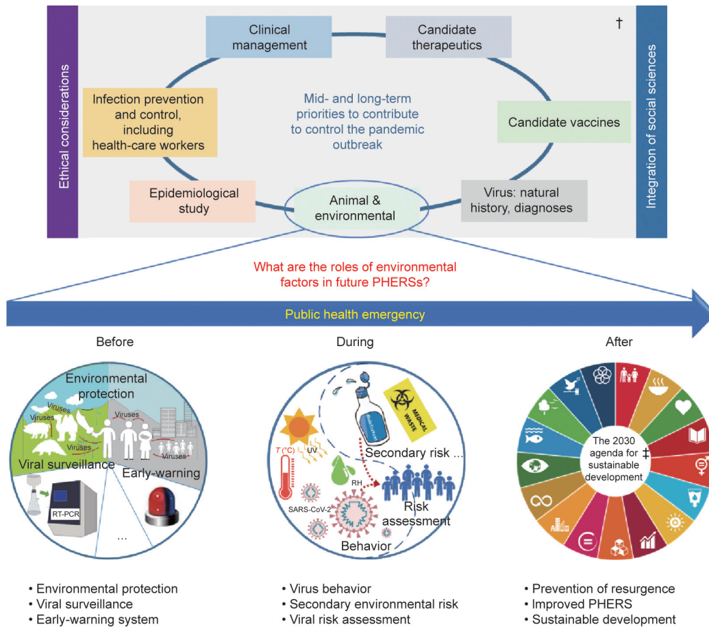
Fig. 1. An illustration of the roles of environmental factors in future PHERSs. Before a pandemic outbreak, environmental and wildlife protection should be strengthened, detailed viral surveillance should be conducted in animals and hotspots, and early-warning systems should be improved to minimize the outbreak of a pandemic. During a pandemic, the impacts of environmental factors on viral behaviors should be studied; also, control measures to minimize secondary environmental risks and timely assessments of viral risks and secondary environmental effects should be undertaken in order to reduce the impacts of the pandemic on human health and ecosystems. After a pandemic, surveillance for viruses and prevention of viral spread should be strengthened, control measures for minimizing secondary environmental risks should be maintained, and scientific prediction capability should be developed in order to respond to the next unexpected resurgence in a timely manner. Meanwhile, the normal life and production of the public should be sustainably restored (sources of illustrations: † reproduced from Ref. [3] with permission of WHO; ‡ the 17 goals are from Ref. [4]). T: temperature; RH: relative humidity; UV: ultra violet; RT-PCR: reverse transcription-polymerase chain reaction.
