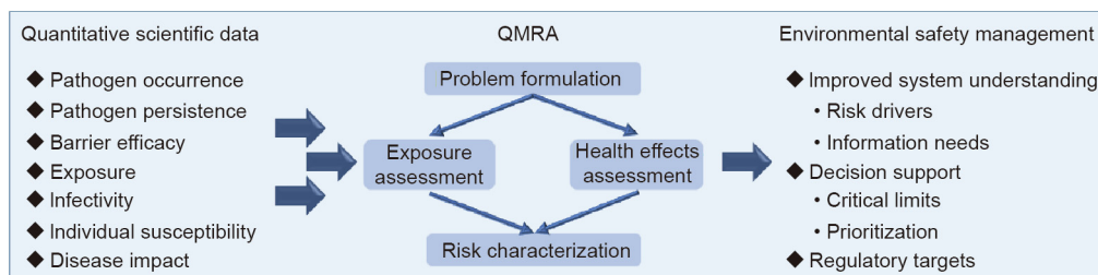
Fig. 3. QMRA: a tool for combining quantitative scientific data related to environmentally relevant disease pathways to support environmental safety management.
