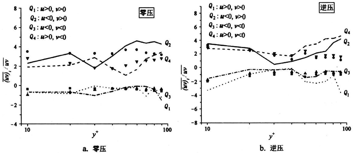
图 3 零压、逆压下 Q_1, Q_2, Q_3, Q_4 对雷诺应力的贡献 Fig.3 Contribution of Q_1, Q_2, Q_3, Q_4 to Reynolds-stress
