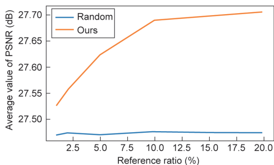
Fig. 8. Plots show the effectiveness of our engram association module.
