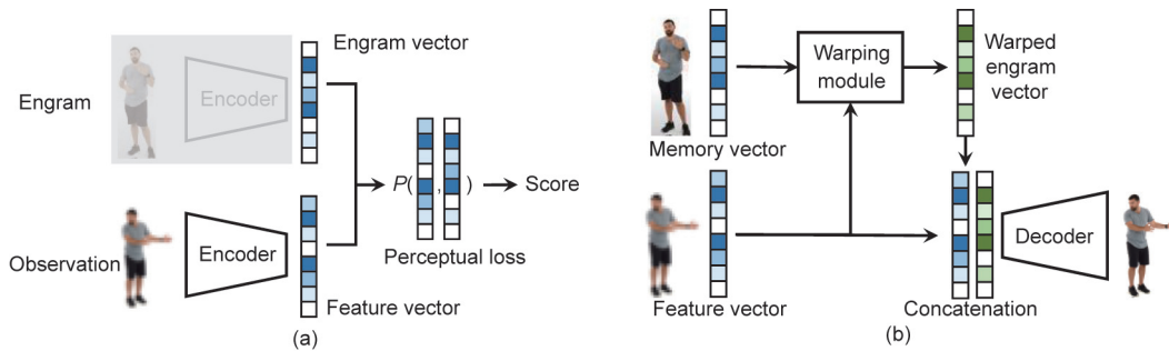
Fig. 4. Network structure of two sub-modules in the feedback pathway. (a) Association module for engram extraction; (b) synthesis module. P : perceptual loss.
