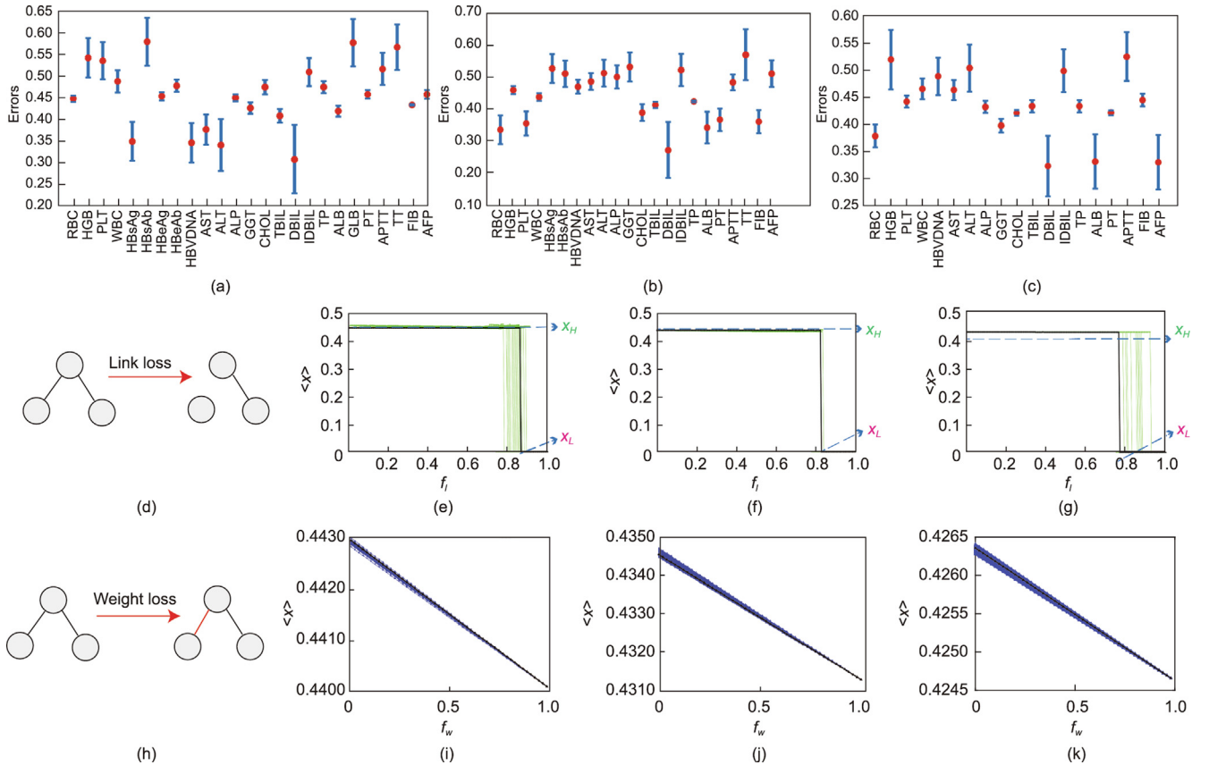
Fig. 3. Dynamics fitting and network resilience in the CHB, LC, and HCC states. (a–c) We fitted dynamics and estimated the unknown parameters I_{i,k} and R_{i,k} for CHB, LC, and HCC, when the parameters n = 2 and a = -1 . Red dots indicate the real values of the items, and blue lines show the fitted errors. (d) We tested the resilience of networks against the random disappearance of correlations with a proportion f_l . (e) Average levels of test items in the CHB network vs f_l across 100 realizations (we highlight the analytical solution in black). At a critical fraction f_l^c , the system undergoes a vertical drop, where, in addition to the desired state ( x_H ), an undesired state emerges ( x_L ). (f–g) Similar results are observed in the LC and HCC networks. (h) We tested the resilience of networks against decreasing correlations on average to a fraction f_w of their original value, simulating a global change in the physical conditions of patients. (i) Similar simulations characterize the system's response to global perturbations f_w . (j) In the LC state, even if physicians perform antiviral treatment on patients, the condition will still deteriorate. (k) Similarly, the efficiency of antiviral treatment for patients with HCC is minimal.
