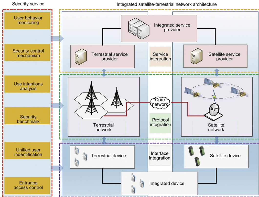
Fig. 1. Integration architecture of the satellite-terrestrial network toward 6G.
