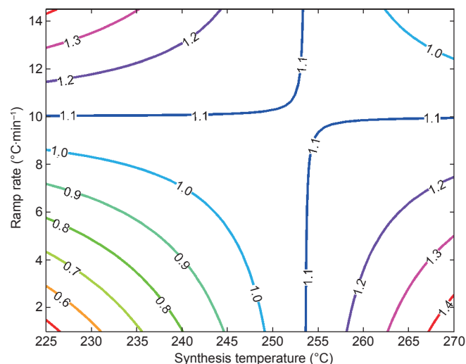
Figure 4. Contour plot obtained from statistical model. CO oxidation activity at 200 °C ( \text{mL}\cdot(\text{g}\cdot\text{s})^{-1} ). The hold values were 0.05 \text{mol}\cdot\text{L}^{-1} of surfactant concentration, 0.1 \text{mol}\cdot\text{L}^{-1} of cobalt concentration, R = 2 of molar ratio, and PVP.
