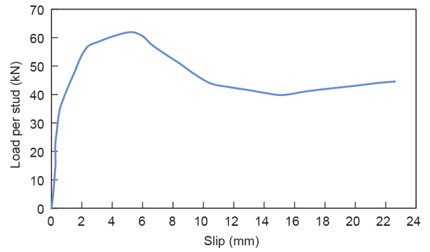
Fig. 8. Load vs. slip curve of the push-off test.
