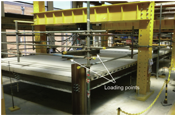
Fig. 11. Loads applied to the internal secondary beam.
