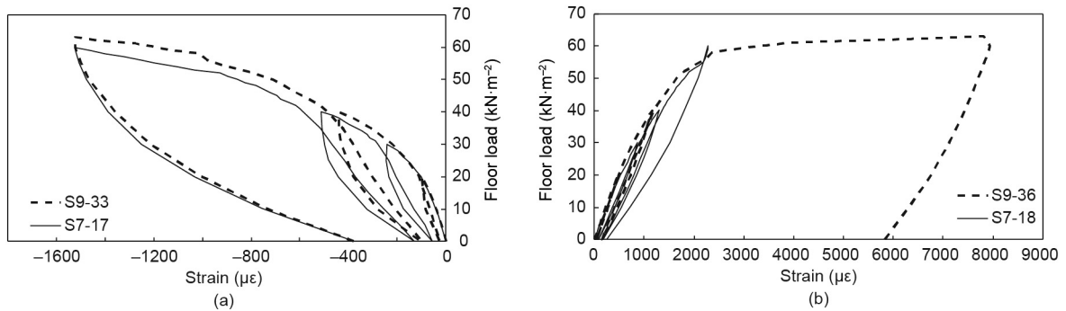
Fig. 18. Typical stress–strain graphs for (a) S7-17/S9-33 and (b) S7-18/S9-36 for loading through the edge beam.
