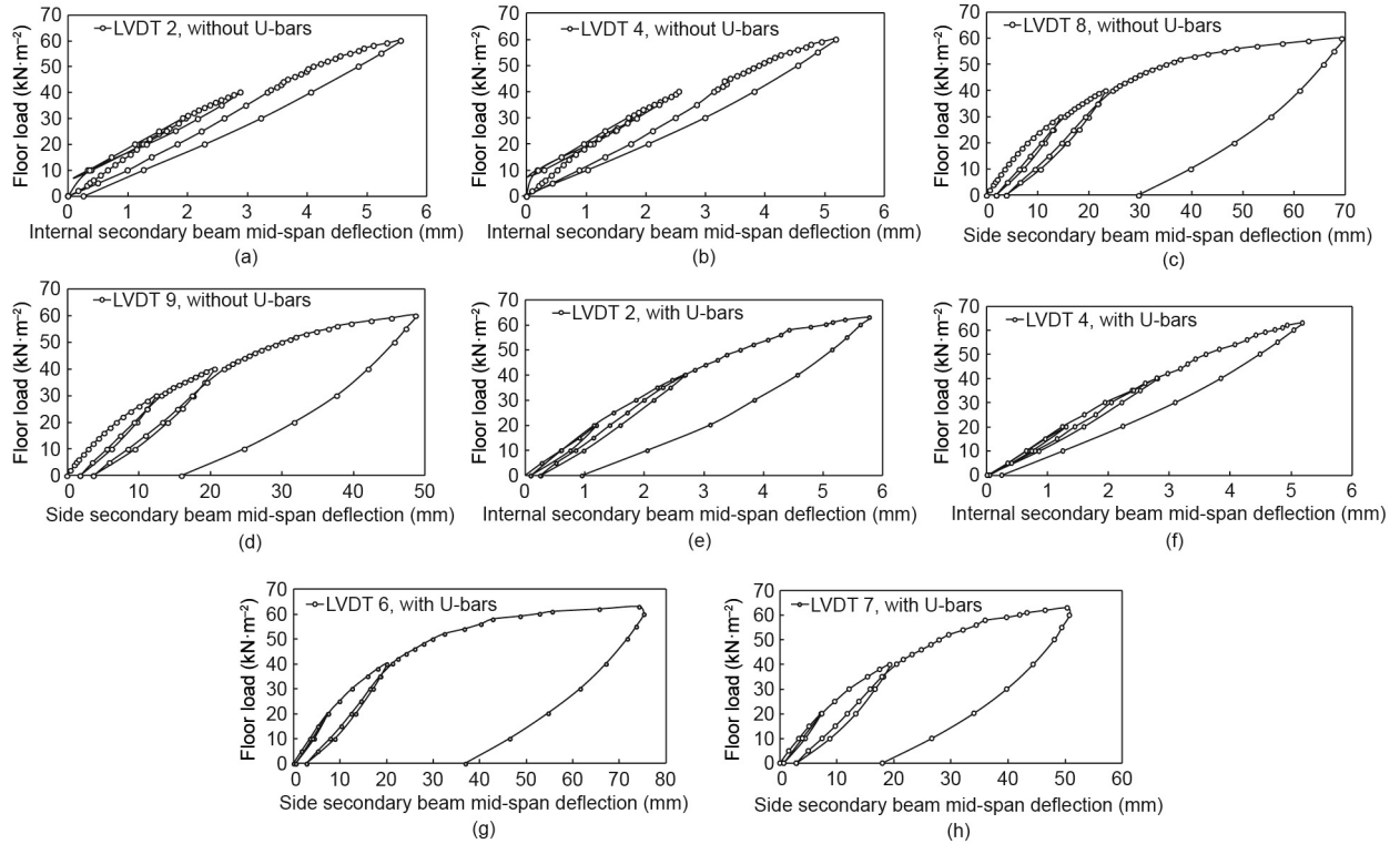
Fig. 17. Graphs for load–deflection relationships at beam mid-span. Tests on edge beams (a–d) without and (e–h) with the U-bars.
