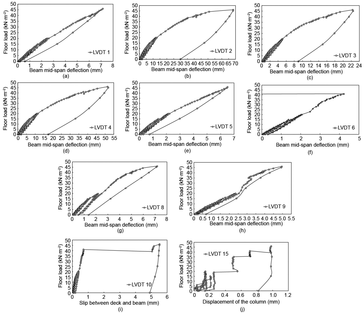
Fig. 13. Typical load-vertical displacement at beam mid-span: (a) LVDT 1; (b) LVDT 2; (c) LVDT 3; (d) LVDT 4; (e) LVDT 5; (f) LVDT 6; (g) LVDT 8; (h) LVDT 9; (i) LVDT 10; (j) LVDT 15.
