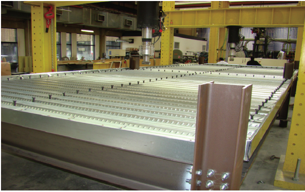
Fig. 4. Steel decking and shear connector arrangement.
