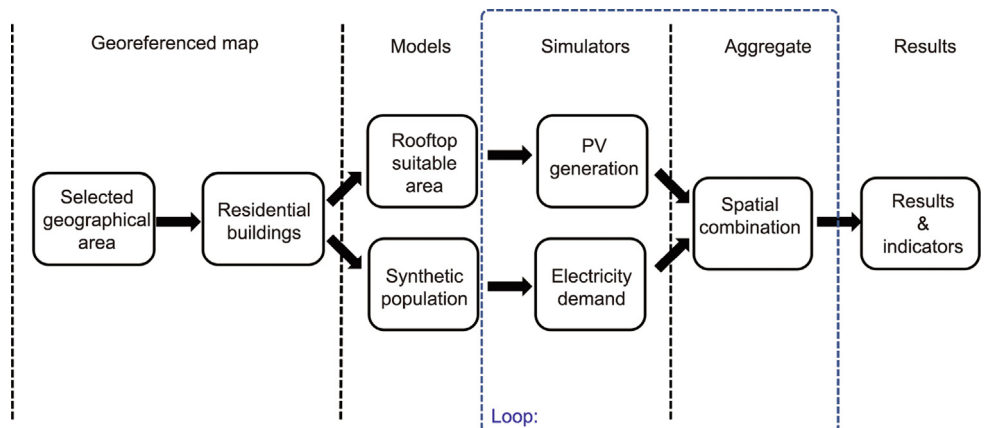
Fig. 2. Orchestrator work-flow.
