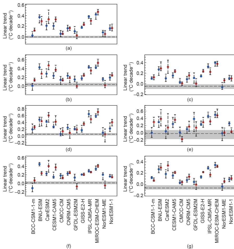
Fig. 3. Weighted linear trend ( ^{\circ}\text{C-decade}^{-1} ) in the models for the (a) globe, (b) NH, (c) SH, (d) NH land, (e) SH land, (f) NH ocean, and (g) SH ocean from 2001 to 2013 under RCP4.5 (blue circles) and RCP8.5 (red circles). The dashed line indicates the value of the trend from HadCRUT4 reanalysis, and the shaded area covers the 50% confidence interval. Error bars show the 50% confidence interval for each model.
