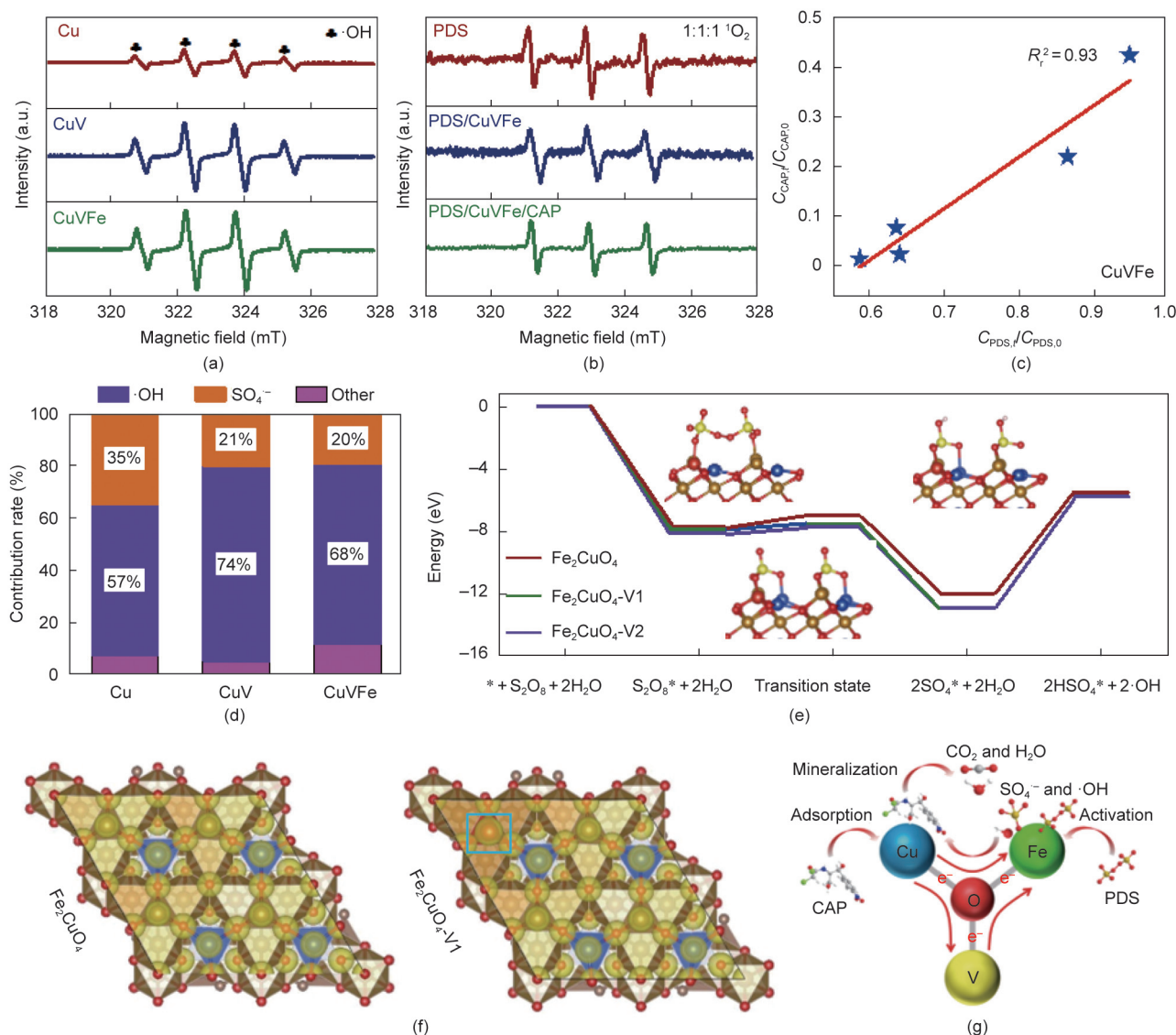
Fig. 4. (a) EPR spectra using DMPO as trapping reagents for \bullet\text{OH} and \text{SO}_4^{\bullet-} . (b) EPR spectra using TEMP for ^1\text{O}_2 . (c) The linear relationship of PDS activation and CAP removal efficiency. (d) The contribution rate of different ROS by Cu, CuV, and CuVFe materials. (e) Energy profiles in different structures from material/ \text{S}_2\text{O}_8 systems to material/ 2\text{HSO}_4 systems. Insert map representing \text{Fe}_2\text{CuO}_4\text{-V1} structure. (f) The corresponding charge-density wave for \text{Fe}_2\text{CuO}_4 and \text{Fe}_2\text{CuO}_4\text{-V1} . (g) The catalytic mechanism of CuVFe for PDS activation and organic pollutant degradation in different elements. R^2 represented the fit degree of a linear regression model.
